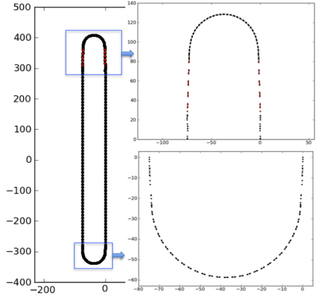
Figure 6: Storage ring geometry. The entire ring is on the left while the subfigures on the right show zoomed images of the areas highlight by blue boxes. The red dots represent the injection insertion.
