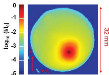
Figure 2: Reconstructed UMER beam profile.
