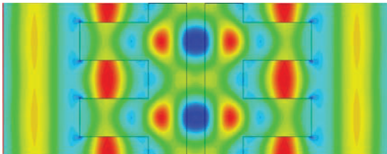
Figure 3: z-component of the electric field distribution in dual-gratings structure.
