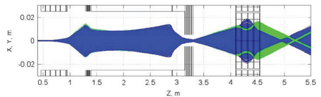
Figure 1: Particle trajectories from solenoid through acceleration section.
